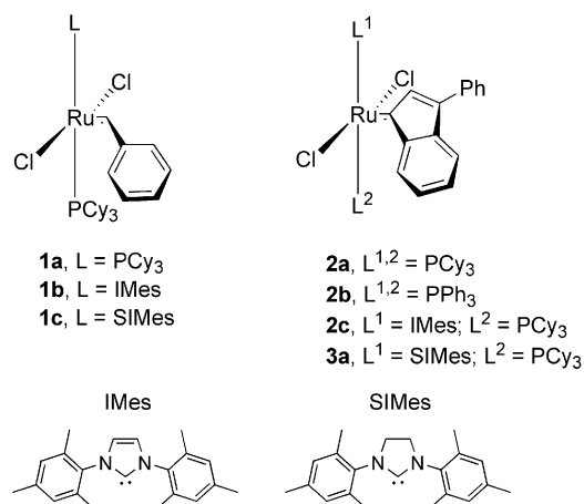
Figure 1. Benzylidene and indenylidene ruthenium complexes.
