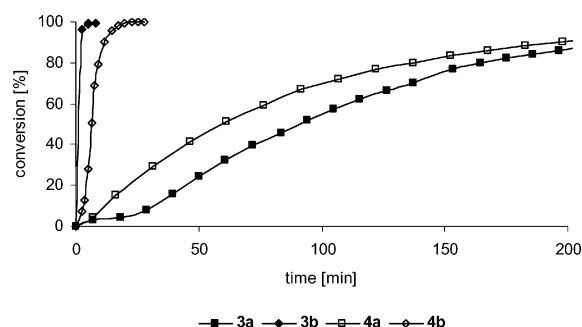
Figure 8. ROMP of 1,5-cyclooctadiene ( 18 ), catalysts 3a–b and 4a–b . Catalyst/monomer ratio 1:3000; solvent: CDCl 3 ; temperature: 20 °C; conversion determined by 1 H NMR; lines are intended as visual aids.
