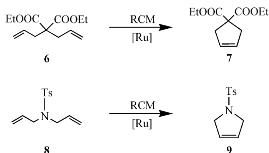
Scheme 1. Representative Ring-Closing Metathesis reactions.
