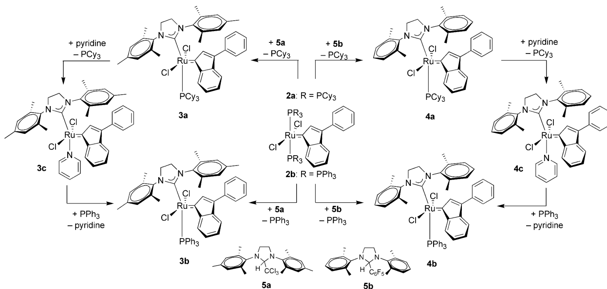
Figure 2. Synthetic pathways to 2 nd - and 3 rd -generation indenylidene-Ru metathesis catalysts.
