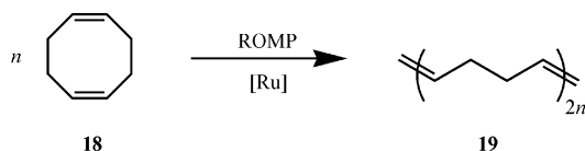
Scheme 2. ROM polymerization of 1,5-cyclooctadiene (COD) ( 18 ).
