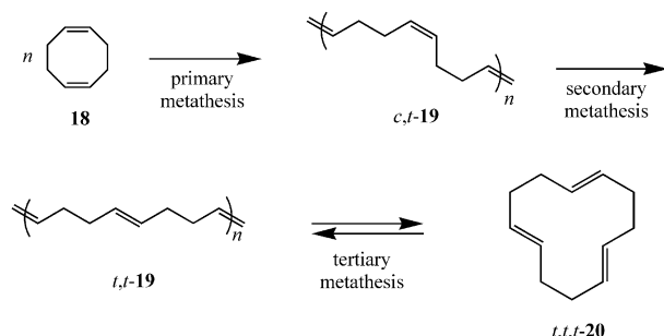
Scheme 3. Formation of CDT ( 20 ) during the ROMP of COD ( 18 ).
