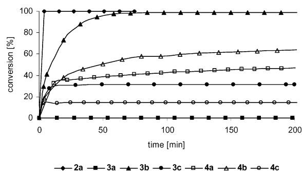
Figure 7. RCM of N,N -diallyltosylamide ( 8 ), catalysts 3a–c , 4a–c . Catalyst/substrate ratio 1:200; solvent: \text{CDCl}_3 ; temperature: 20^\circ\text{C} ; conversion determined by ^1\text{H} NMR; lines are intended as visual aids only.
