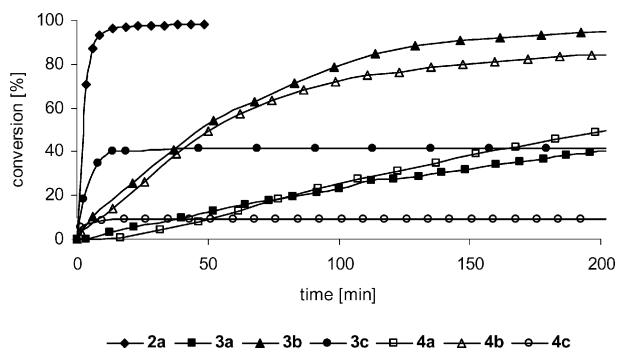
Figure 5. RCM of diethyl diallylmalonate ( 6 ), catalysts 3a–c , 4a–c and 2a . Catalyst/substrate ratio 1:200; solvent: \text{CDCl}_3 ; temperature: 20^\circ\text{C} ; conversion determined by ^1\text{H} NMR; lines are intended as visual aids only.
