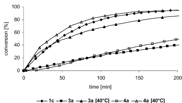
Figure 6. RCM of diethyl diallylmalonate ( 6 ), catalysts 1c , 3a and 4a . Catalyst/substrate ratio 1:200; solvent: \text{CDCl}_3 ; temperature: 20^\circ\text{C} ; conversion determined by ^1\text{H} NMR; lines are intended as visual aids only.
