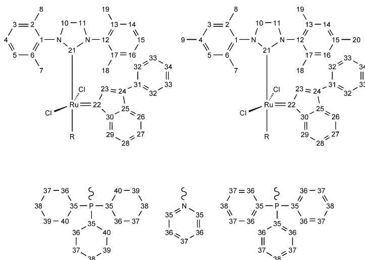
Figure 3. Arbitrary numbering of the common ligands of compounds 3a–c (top, left) and 4a–c (top, right) and of the variable ligand of compounds 3a and 4a (bottom, left), 3c and 4c (bottom middle) and 3b and 4b (bottom right).
