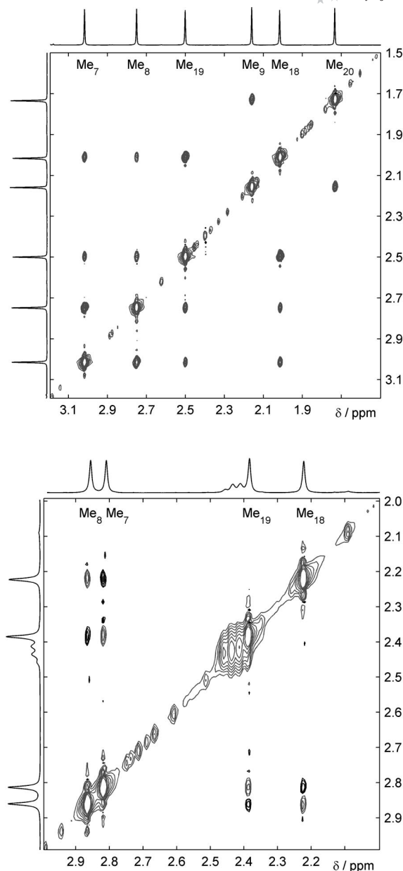
Figure 4. Detail of the 200 ms off-resonance ROESY spectrum demonstrating exchange cross-peaks (grey) indicative of hindered rotations that are slow on the NMR time scale around all possible SIMes bonds in compound 3c (top) while a hindered rotation around the Ru–N(SIME) bond only is observed in compound 4c (bottom). Here, black cross-peaks indicate genuine nOe correlations (Me 7 –Me 18 ; Me 8 –Me 19 ) between methyl groups on both sides of SIME.
